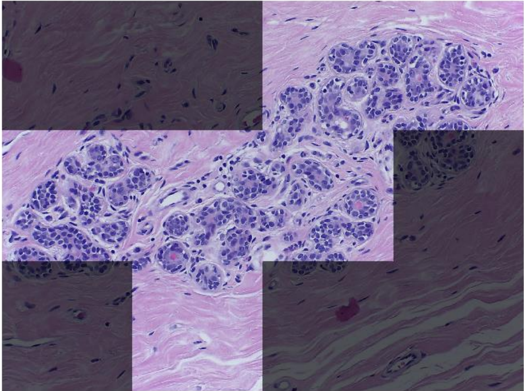
Attention Network
